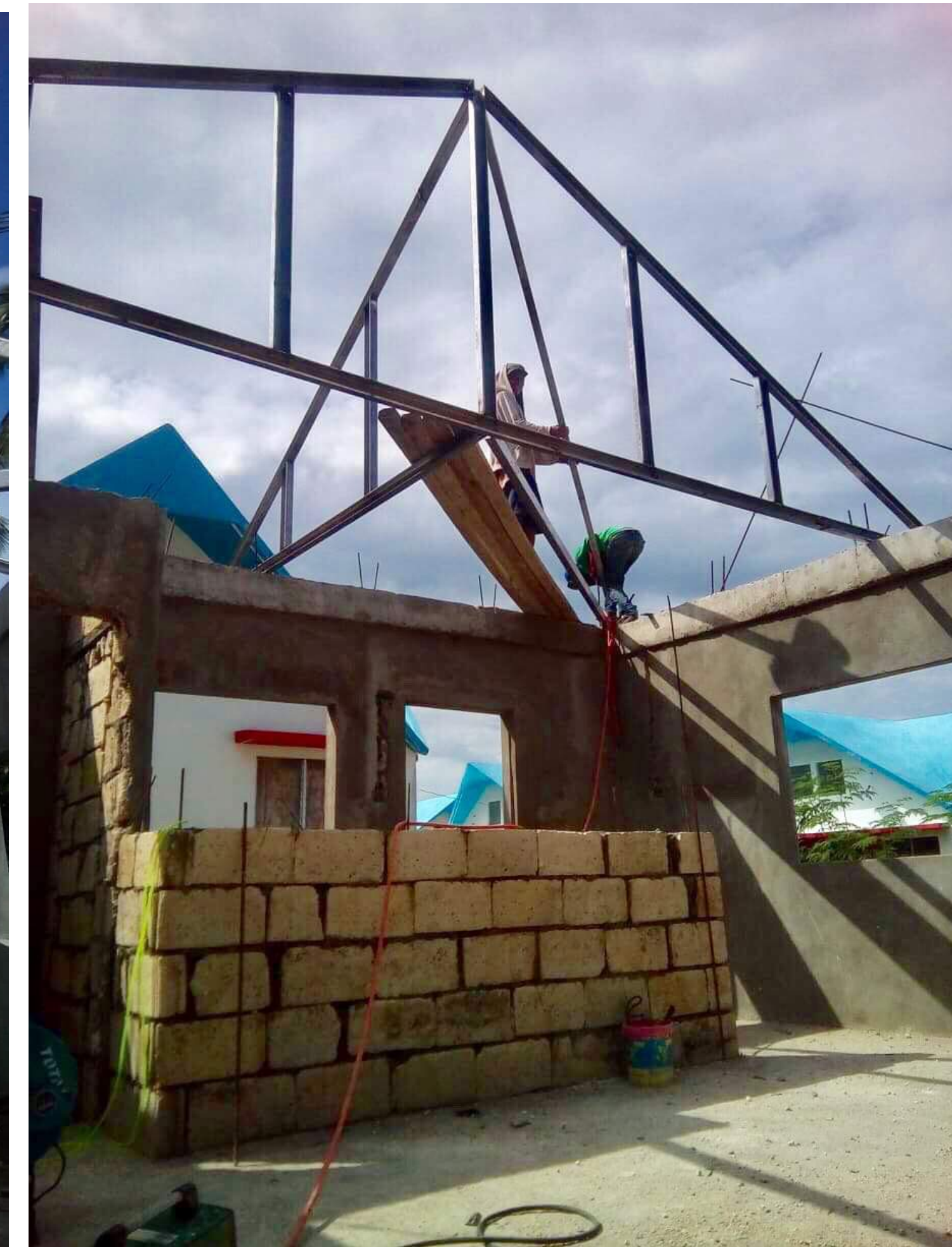
Installation of roof trusses, June 2018
